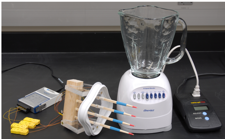
Figure 1: Equipment used in the blender experiment.
