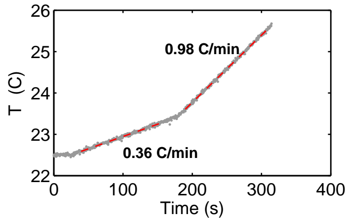
Figure 3: Average thermocouple temperatures as the blender speed increases from puree to liquify with one liter of water in the pitcher. Nominal power consumption is 113 W during puree and 281 W during liquify.
